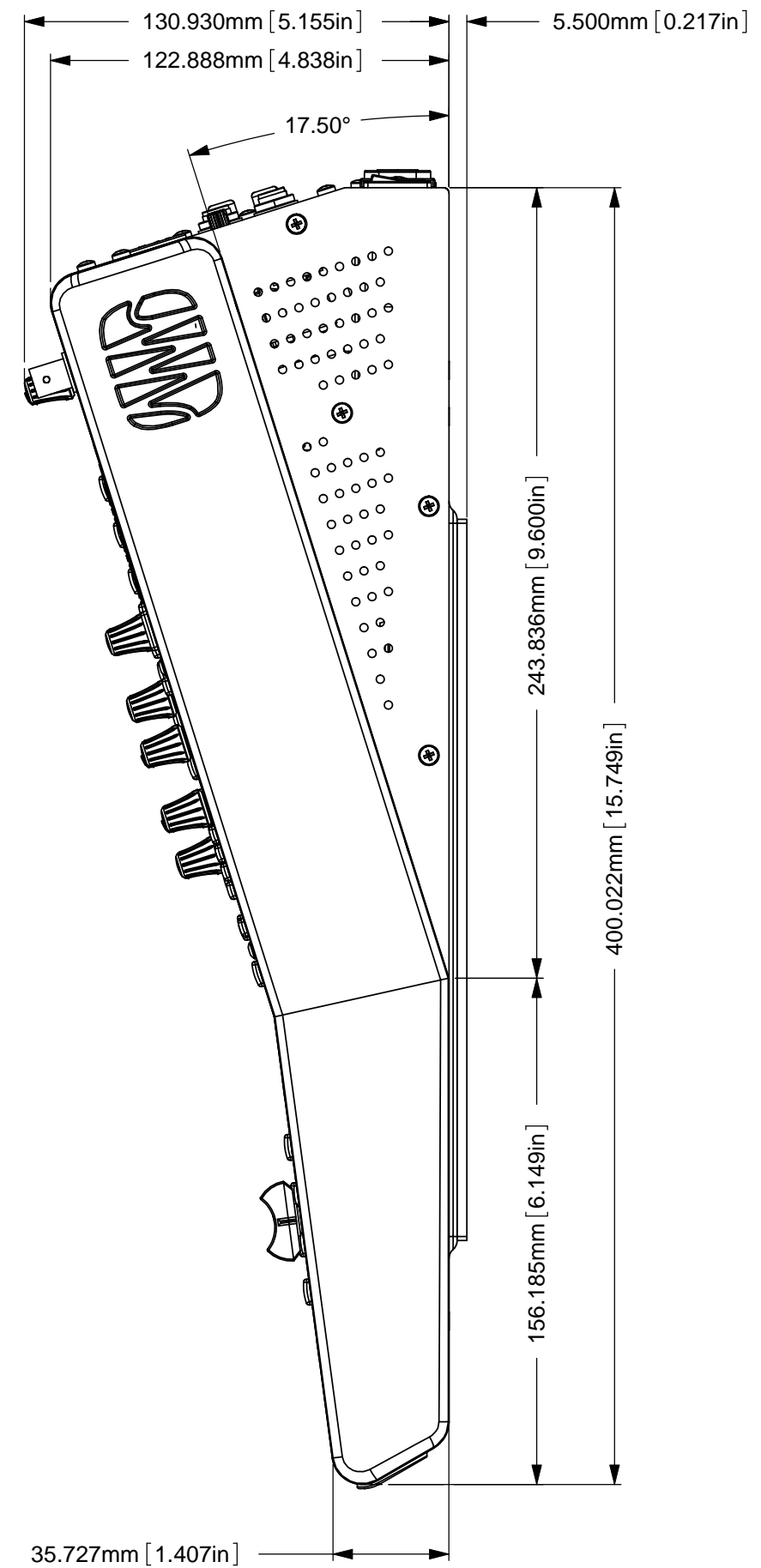
RIGHT VIEW SCALE 1:2
