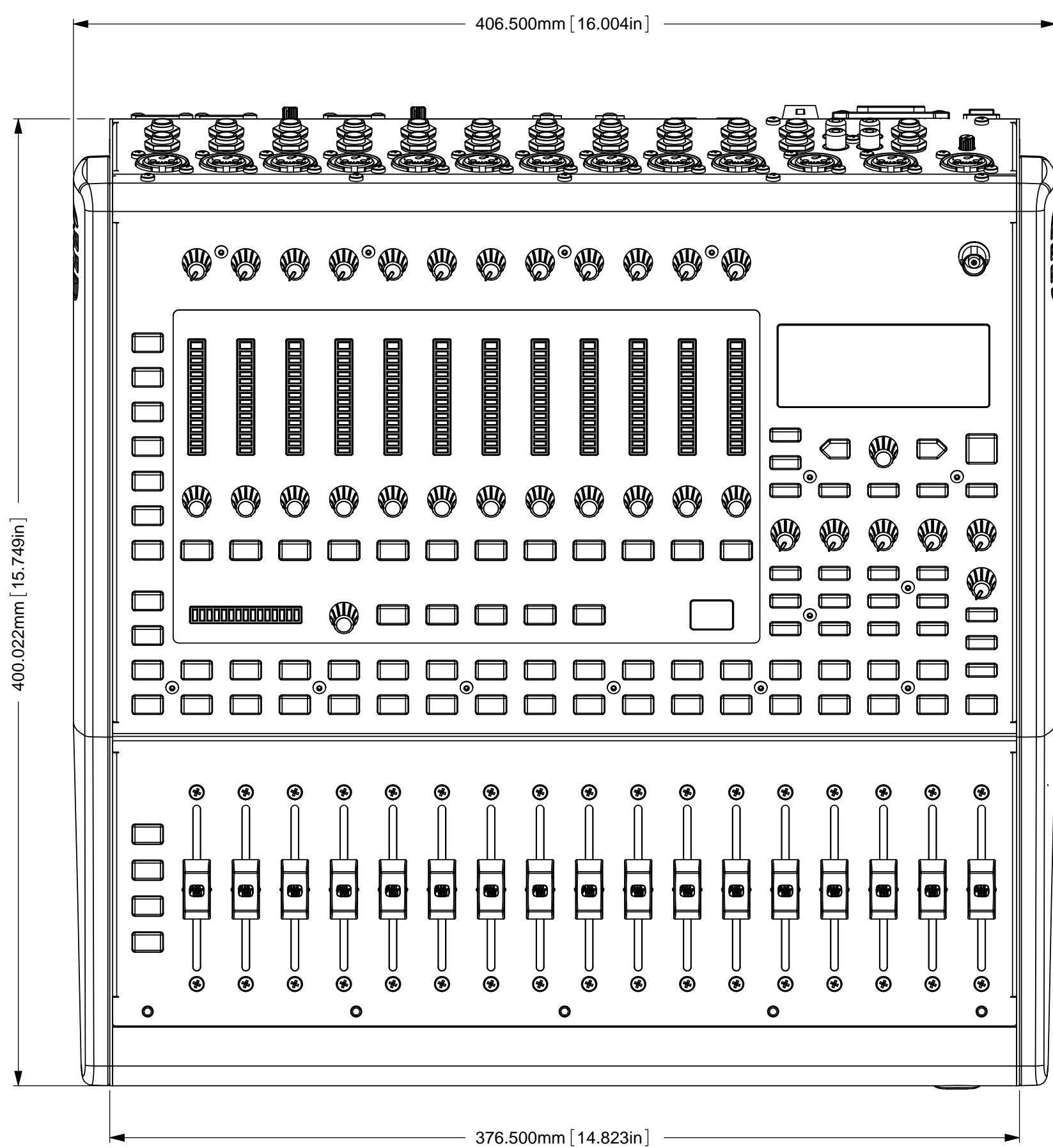
TOP VIEW SCALE 1:2
