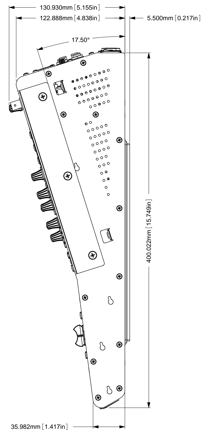
RIGHT VIEW SCALE 1:2
