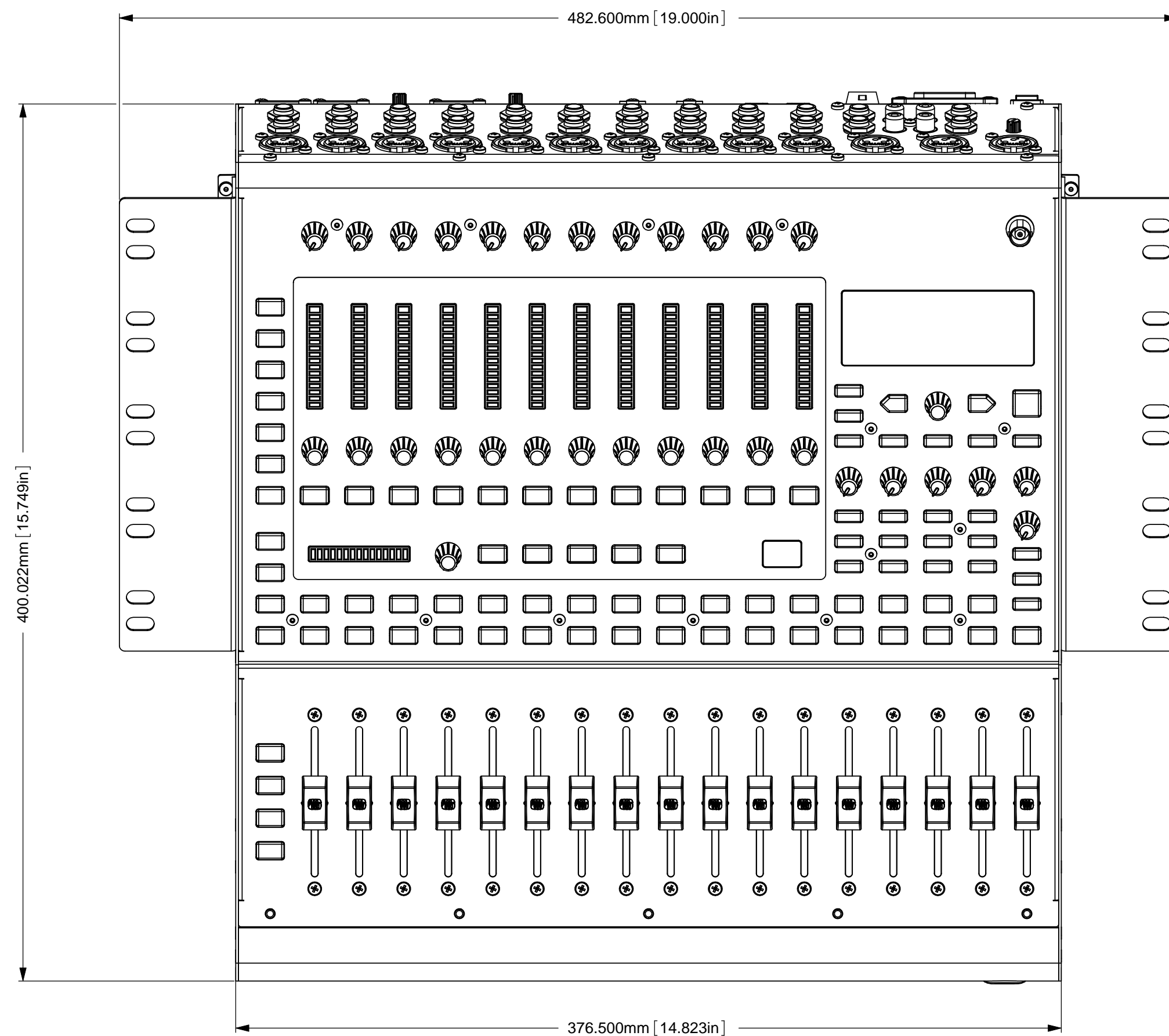
TOP VIEW SCALE 1:2
